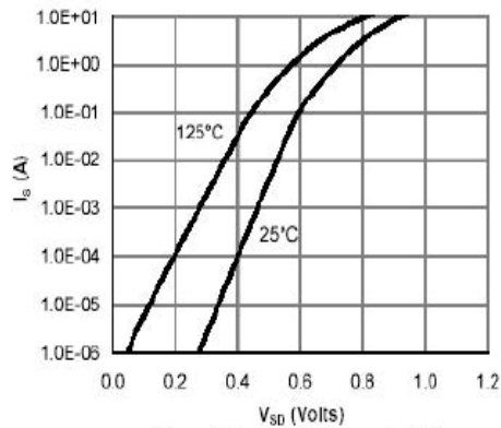
Figure 6: Body-Diode Characteristics
