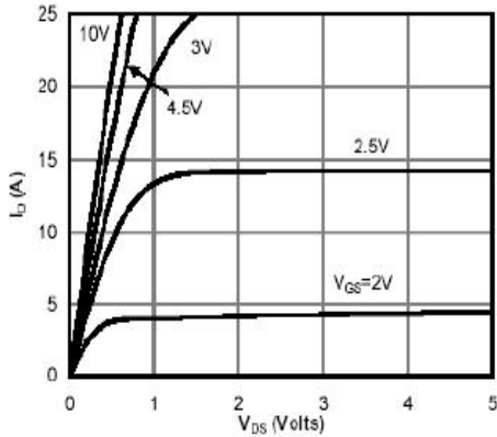
Fig 1: On-Region Characteristics
