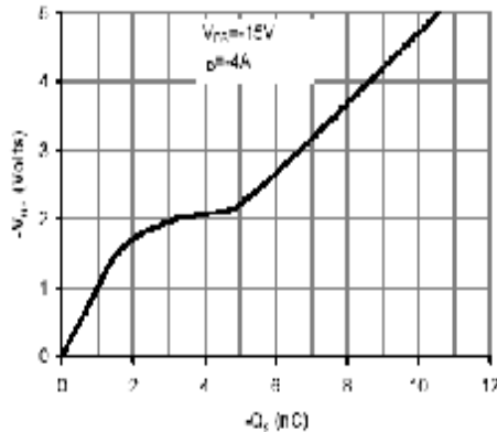
Figure 7: Gate-Charge Characteristics
