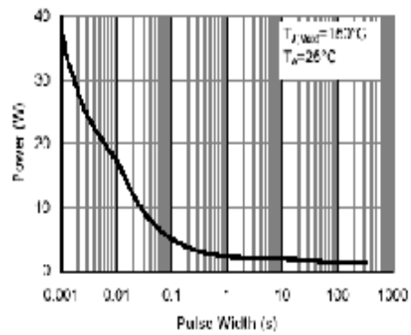
Figure 10: Single Pulse Power Rating Junction-to-Ambient (Note D)
