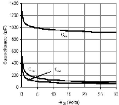
Figure 8: Capacitance Characteristics
