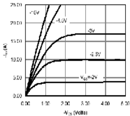
Figure 1: On-Region Characteristics
