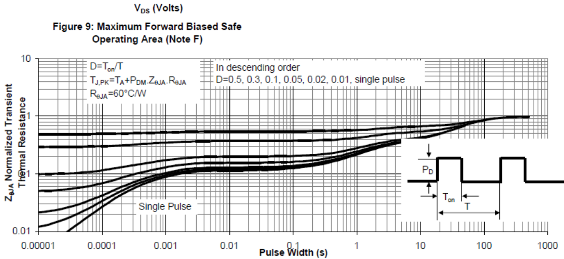
Figure 11: Normalized Maximum Transient Thermal Impedance (Note F)
