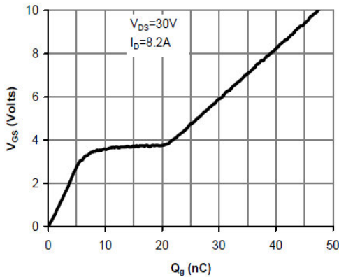
Figure 7: Gate-Charge Characteristics
