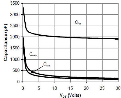
Figure 8: Capacitance Characteristics
