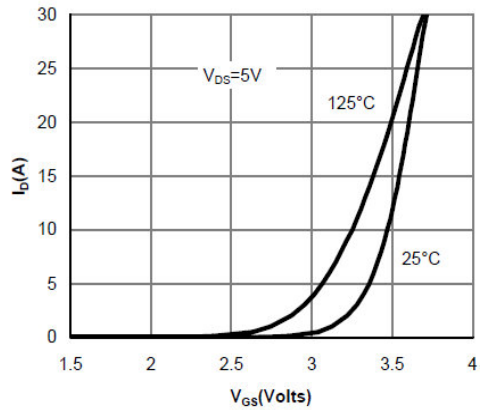
Figure 2: Transfer Characteristics
