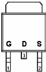
TO-252
